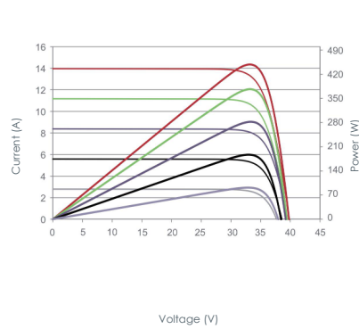
Current-Voltage & Power-Voltage Curves (435W)
