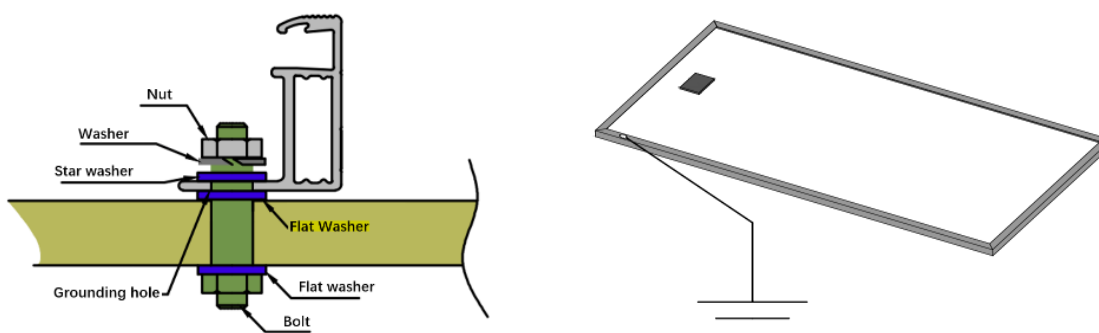
Fig. 12 Ground connection of PV modules
